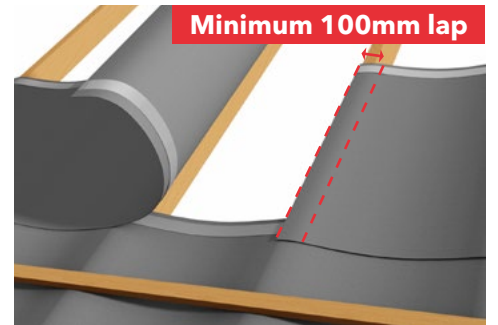
fig 4: Vertical laps
