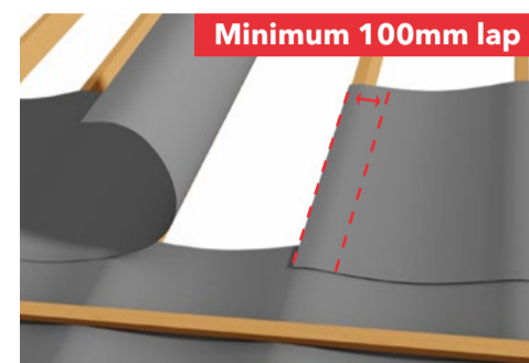
fig 4: Vertical laps
