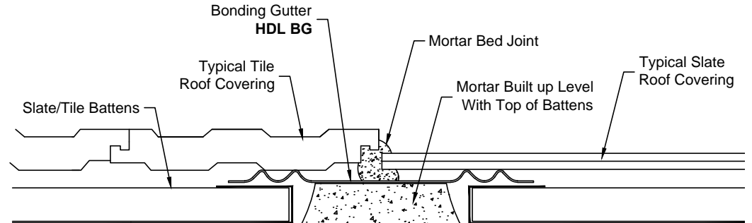
TYPICAL CROSS SECTION - FIRE BREAK DETAIL
