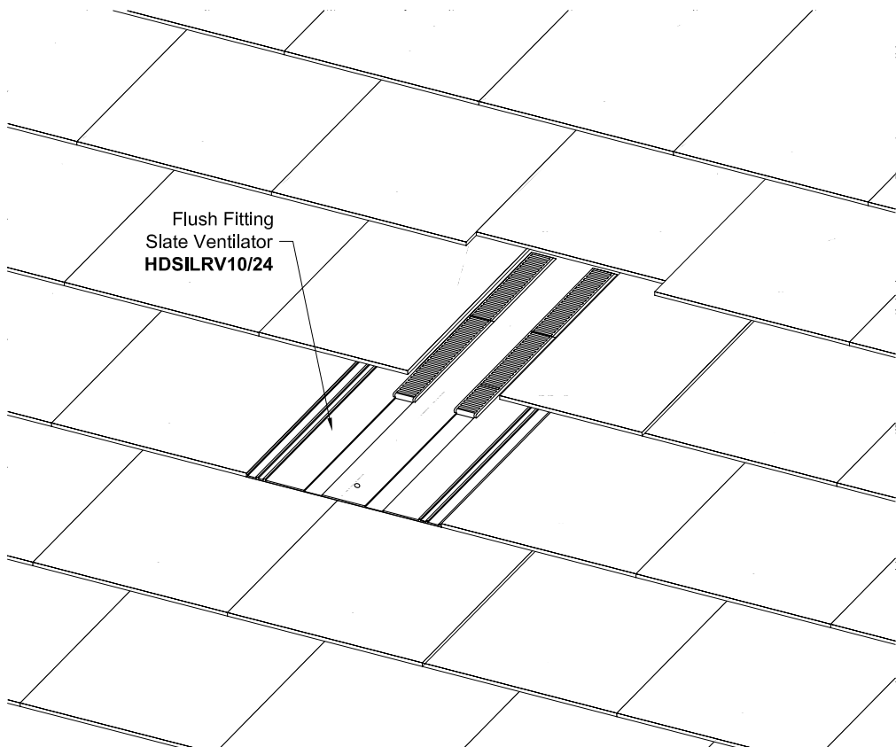
TYPICAL ROOF DETAIL
